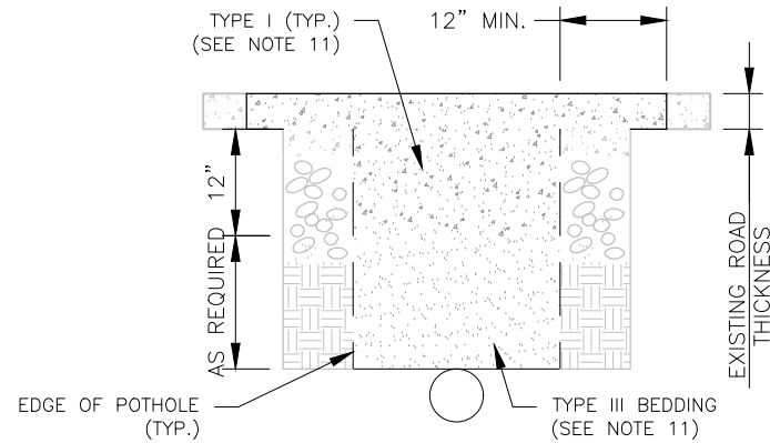
GRAVEL SURFACE REPAIR
