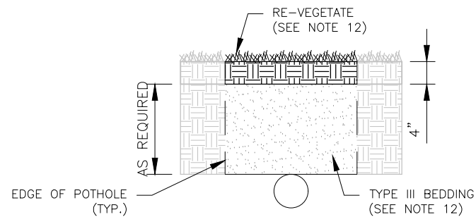
VEGETATIVE SURFACE REPAIR
