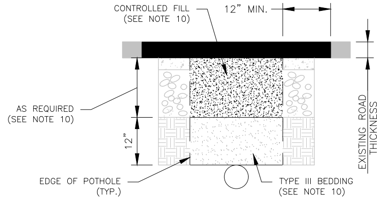
ASPHALT SURFACE REPAIR
