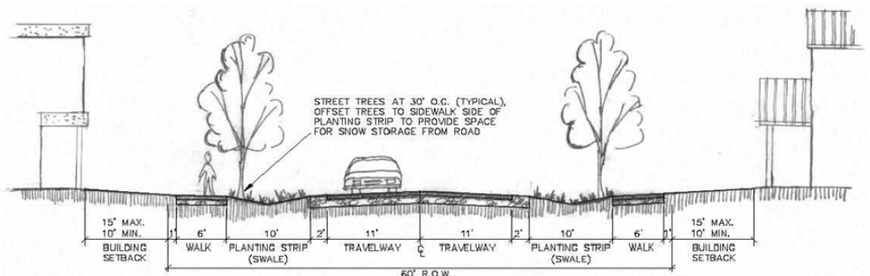
TYPICAL INTERIOR STREET CROSS SECTION
